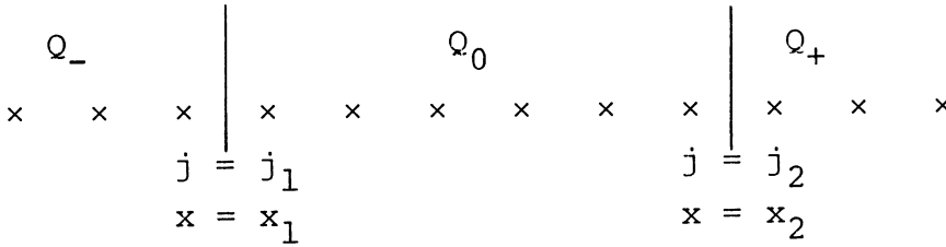
FIGURE 5 Two-interface model
